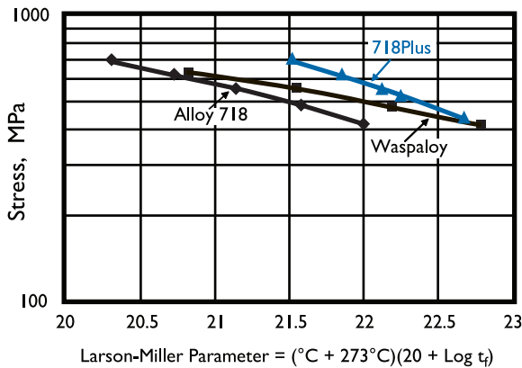
Larson-Miller Plot of Stress Rupture Life of Alloy 718Plus in Comparison with Alloy 718 and Waspaloy
