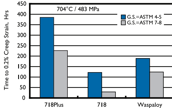
Comparison of Creep Resistance of ATI 718Plus Alloy with Alloy 718 and Waspaloy (Samples from 150 - 200 mm Round Production Billets)
