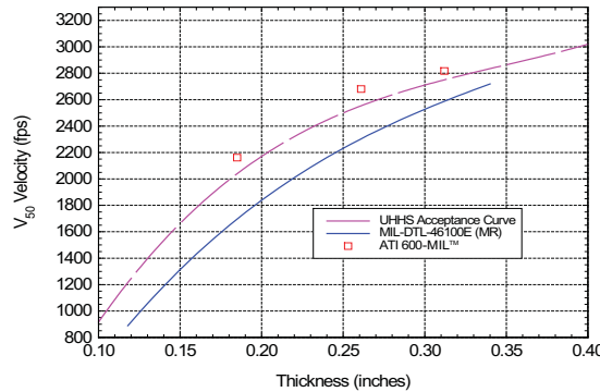
Typical ballistic results of ATI 600-MIL® against 30 Cal. AP M2 projectile. (Courtesy of Army Research Labs).
