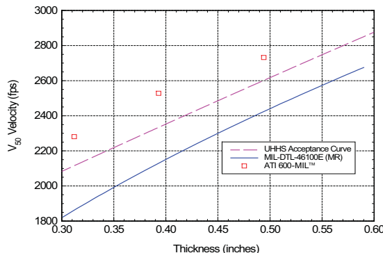
Typical ballistic results of ATI 600-MIL® against 50 Cal. AP M2 projectile. (Courtesy of Army Research Labs).
