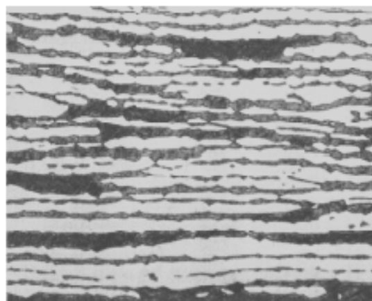
Duplex microstructure of AL 2205™ alloy. The ferrite phase appears darker than the austenite due to KOH etch. The ferrite content is 40% in this sample.
