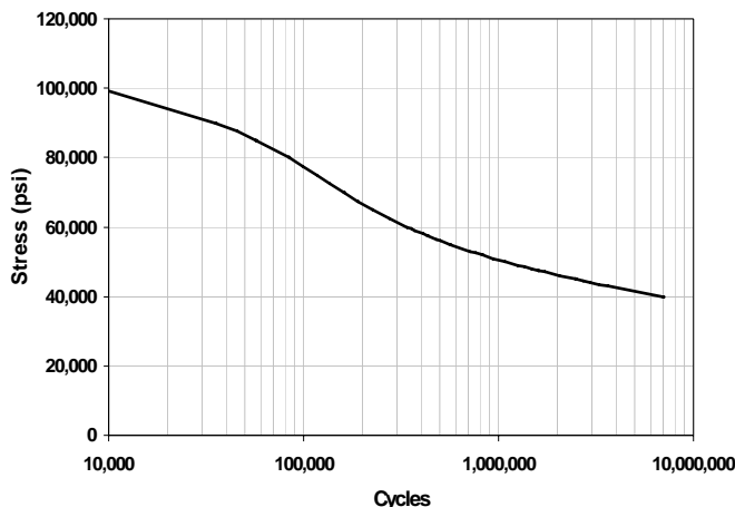
AL 2205™ Alloy Sheet Bending fatigue
