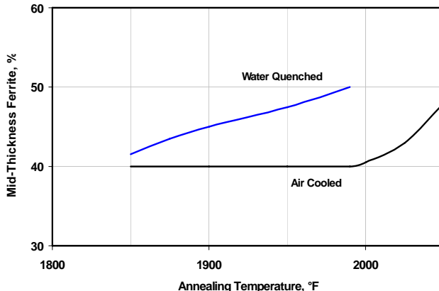
Annealing Response of AL 2205™ Alloy
