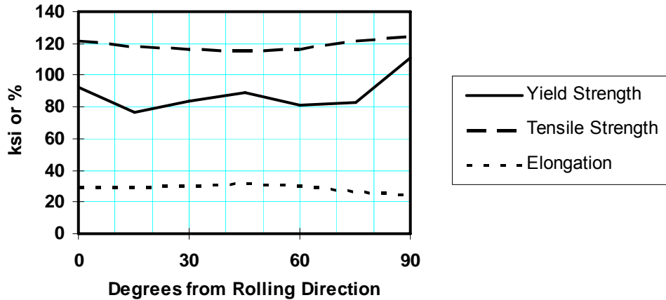
Properties of AL 2205 vs. Orientation
