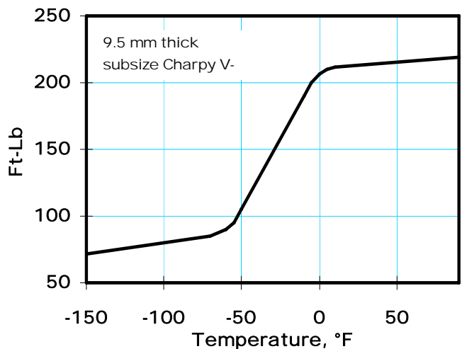
Impact Energy Absorbed vs. Temperature
