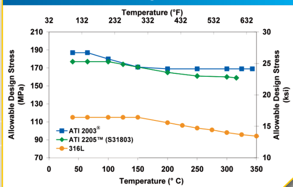
ASME BPV Allowable Design Stresses for Plate
